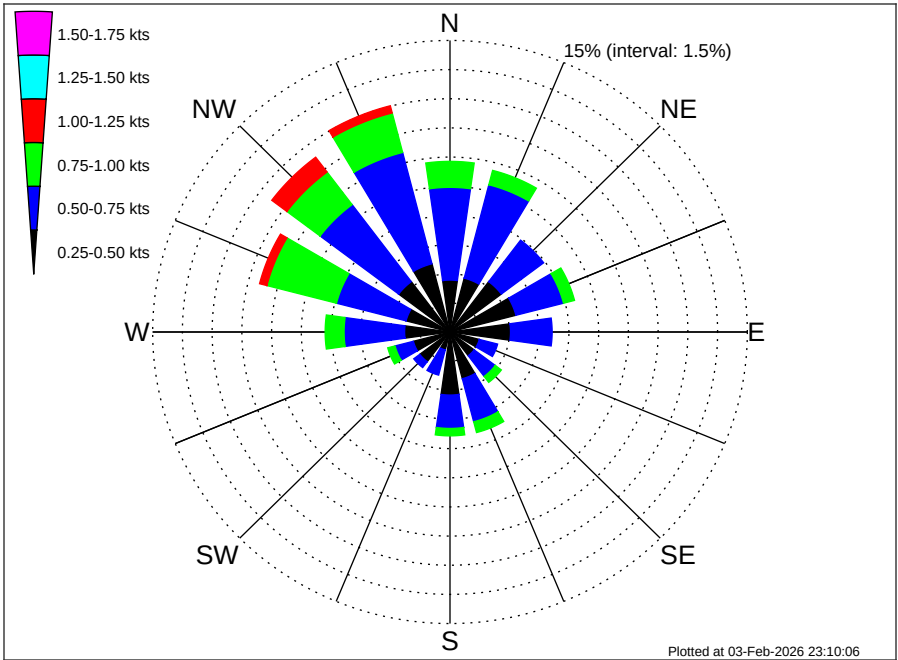
Angola Namibia CRS Mocamedes (BU-MO) Climatological Surface Current Rose for May: 1995 - 2012
