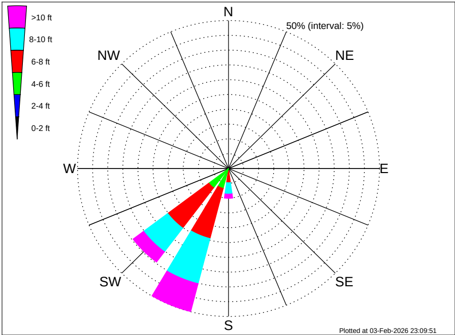
Angola Namibia CRS Mocamedes (BU-MO) Climatological WaveHeight Rose for May: 1979 - 2015
