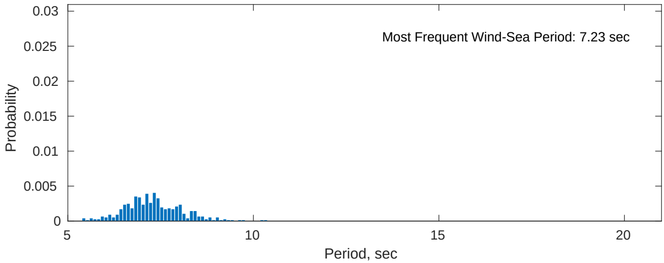
Wind-Sea: 5.61%
