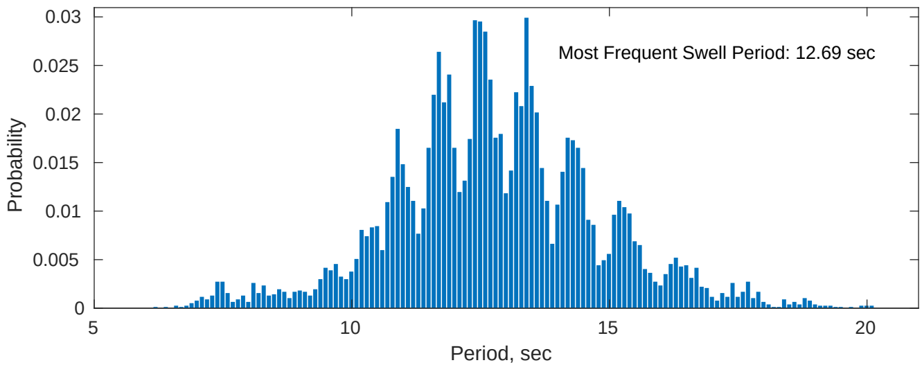
Swell: 94.39%
