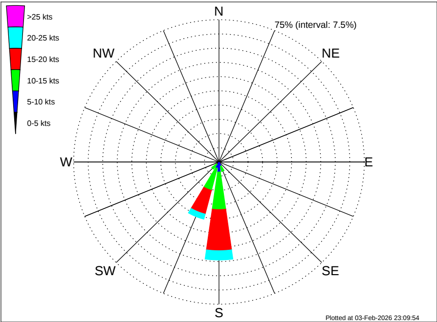
Angola Namibia CRS Mocamedes (BU-MO) Climatological Wind Rose for May: 1979 - 2015
