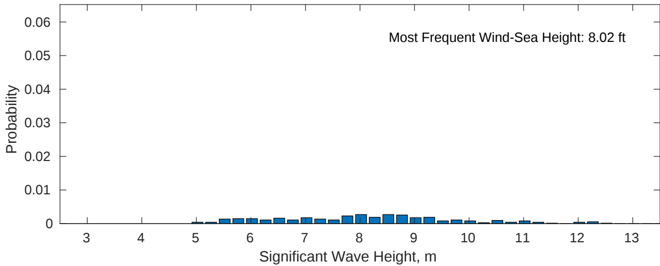
Wind-Sea: 3.55%
