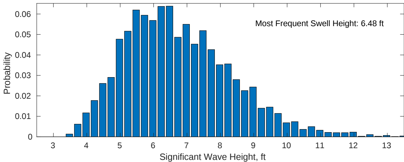
Swell: 96.45%
