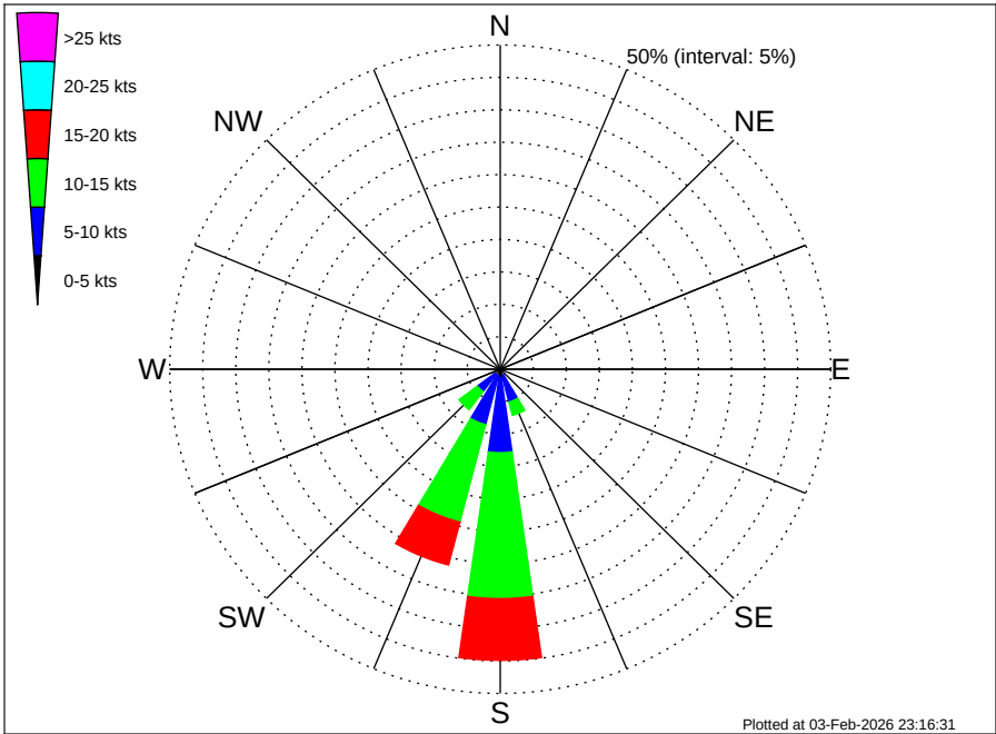
Angola Namibia CRS Mocamedes (BU-MO) Climatological Wind Rose for November: 1979 - 2015
