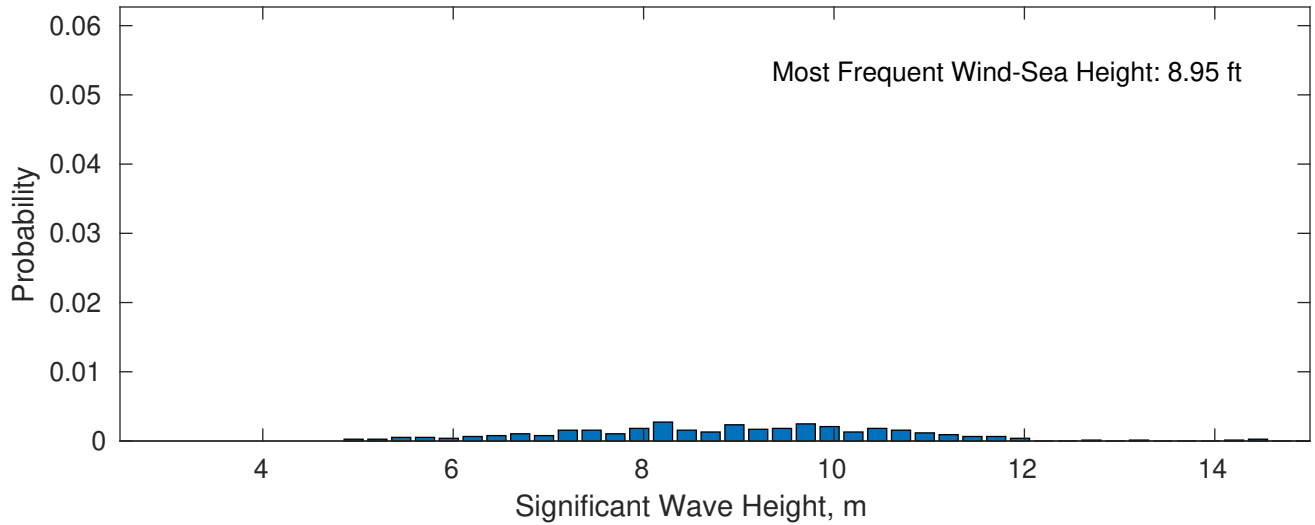
Wind-Sea: 3.71%
