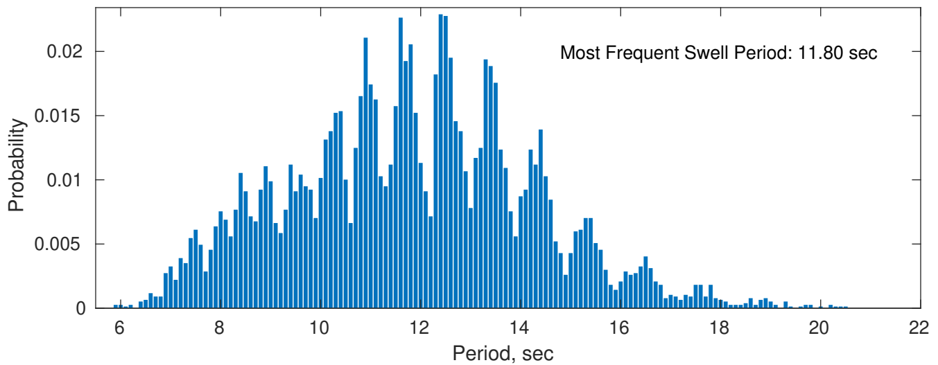
Swell: 96.29%
