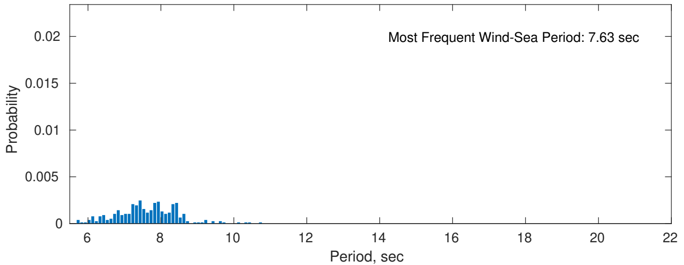
Wind-Sea: 3.71%
