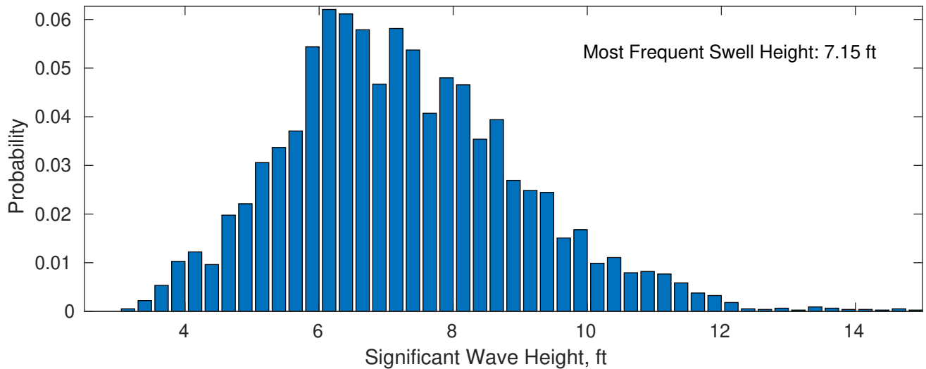
Swell: 96.29%
