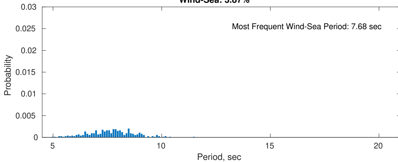
Wind-Sea: 3.87%
