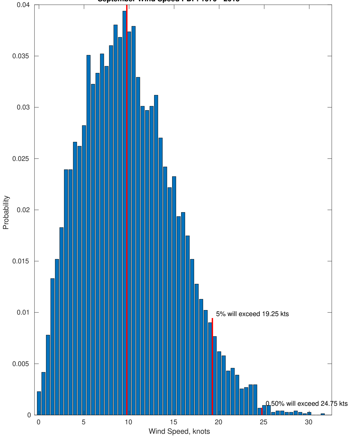
Most Frequent Wind Speed: 9.75 kts September Wind Speed PDF: 1979 - 2015
