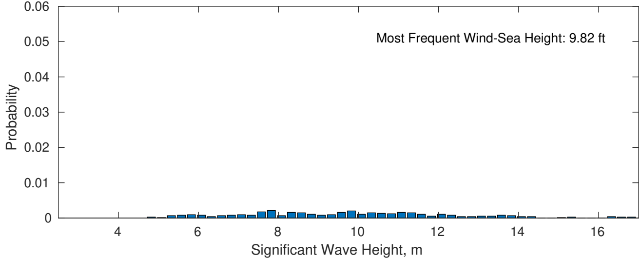
Wind-Sea: 3.87%
