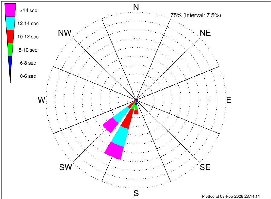
Angola Namibia CRS Mocamedes (BU-MO) Climatological WavePeriod Rose for September: 1979 - 2015
