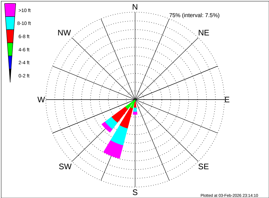
Angola Namibia CRS Mocamedes (BU-MO) Climatological WaveHeight Rose for September: 1979 - 2015
