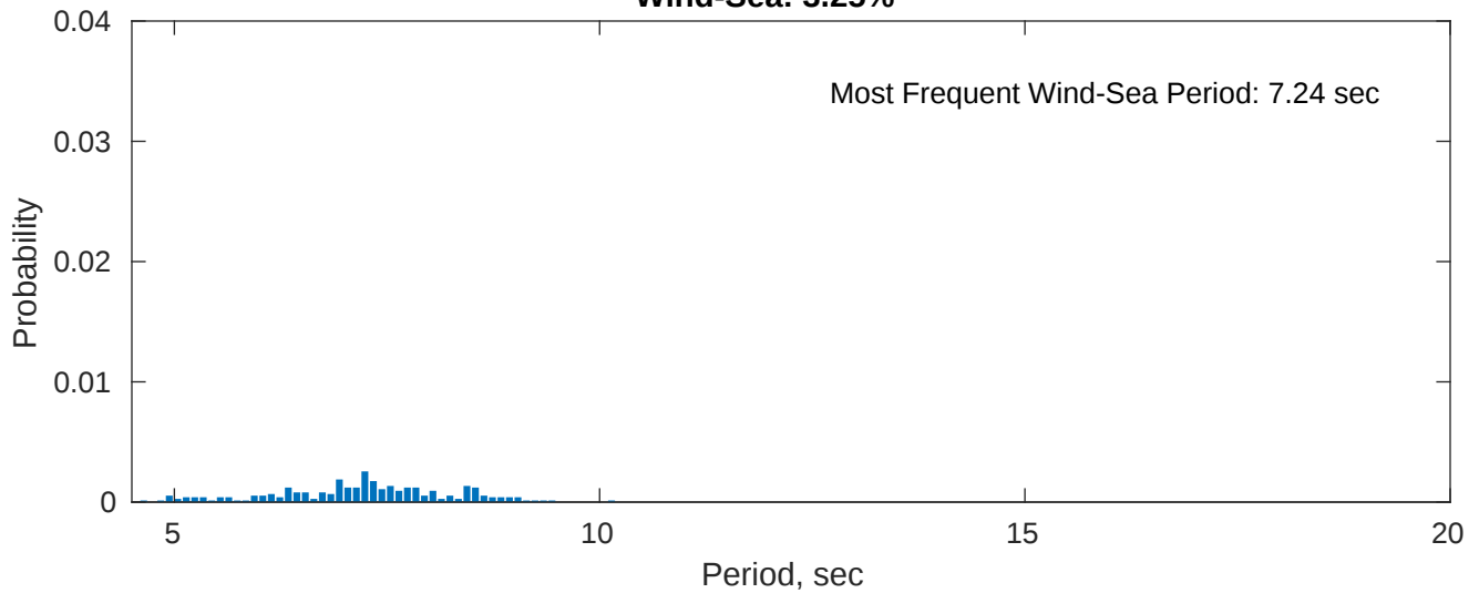
Wind-Sea: 3.25%
