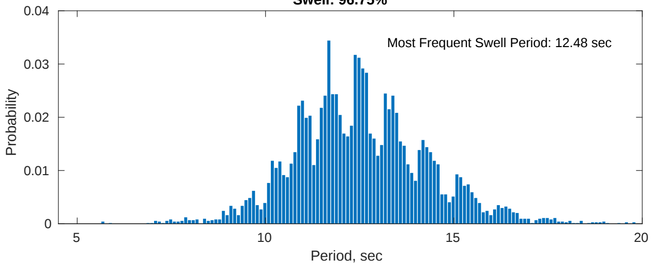
Swell: 96.75%
