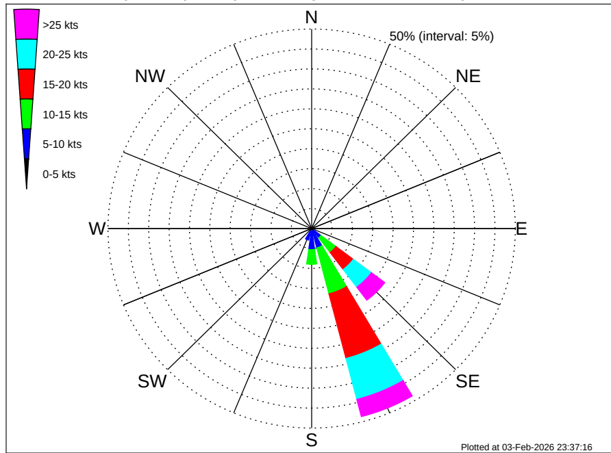
Angola Namibia CRS Oranjemund (BU-OR) Climatological Wind Rose for April: 1979 - 2015
