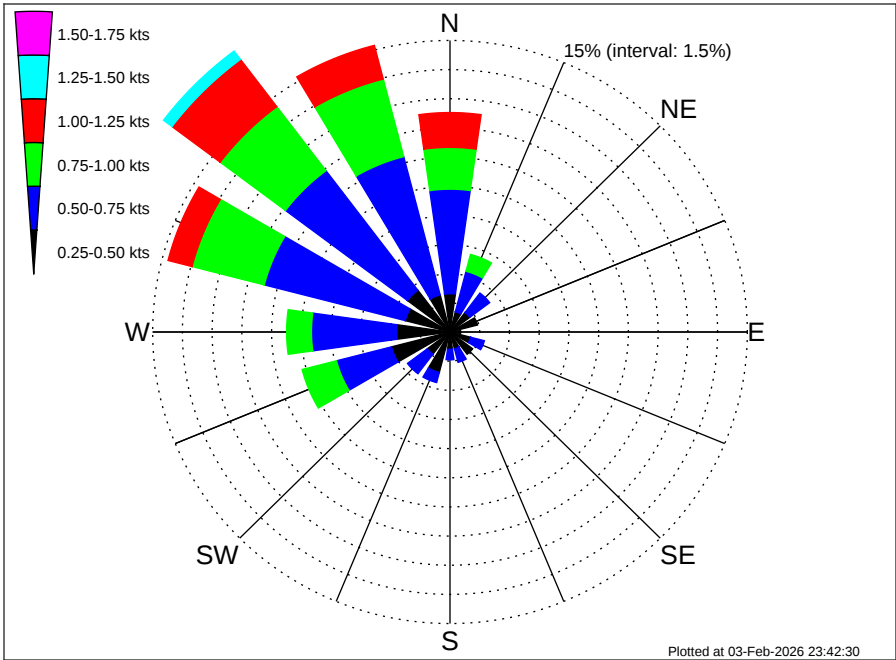
Angola Namibia CRS Oranjemund (BU-OR) Climatological Surface Current Rose for August: 1995 - 2012
