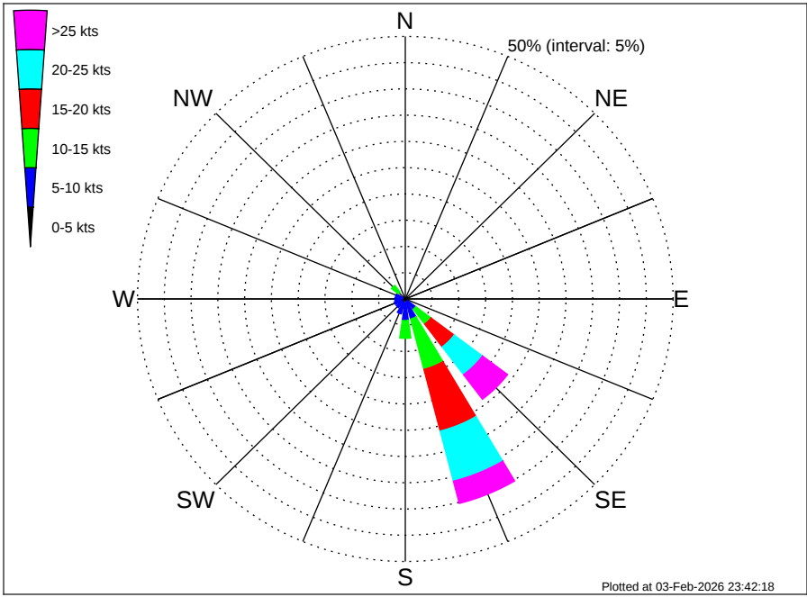
Angola Namibia CRS Oranjemund (BU-OR) Climatological Wind Rose for August: 1979 - 2015
