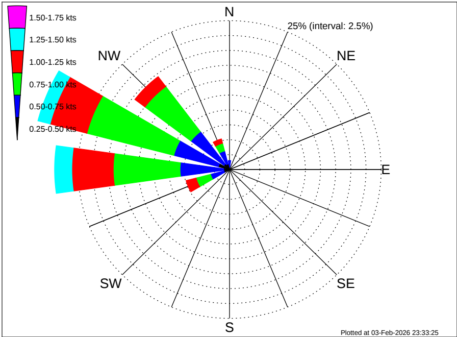
Angola Namibia CRS Oranjemund (BU-OR) Climatological Surface Current Rose for January: 1995 - 2012
