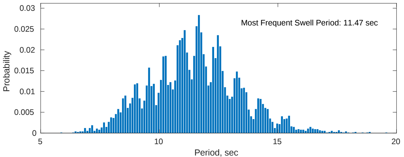
Swell: 88.87%
