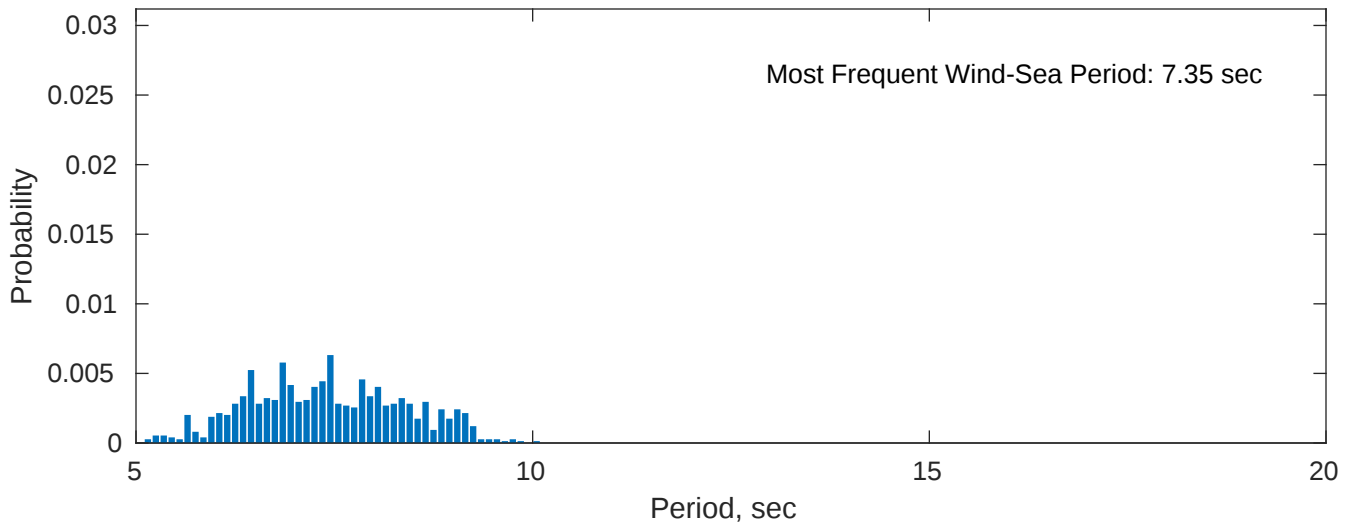
Wind-Sea: 11.13%
