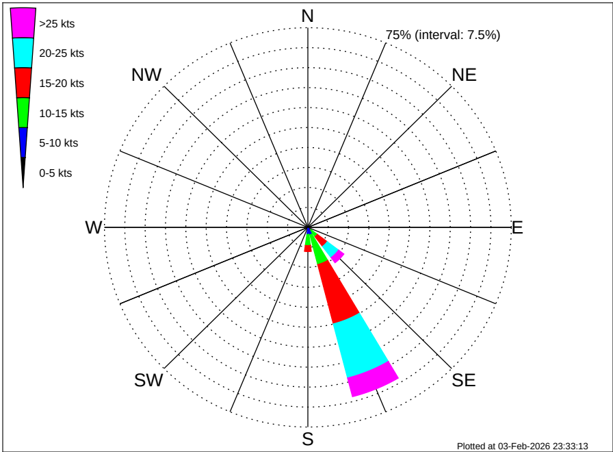
Angola Namibia CRS Oranjemund (BU-OR) Climatological Wind Rose for January: 1979 - 2015
