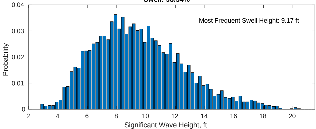
Swell: 98.54%
