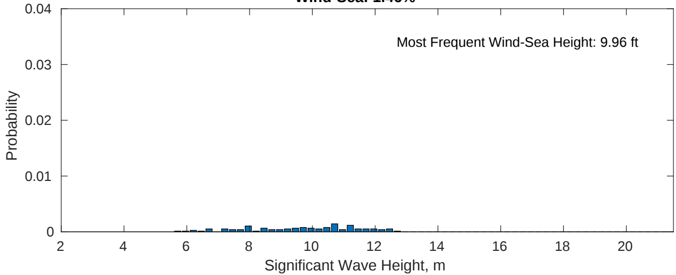
Wind-Sea: 1.46%
