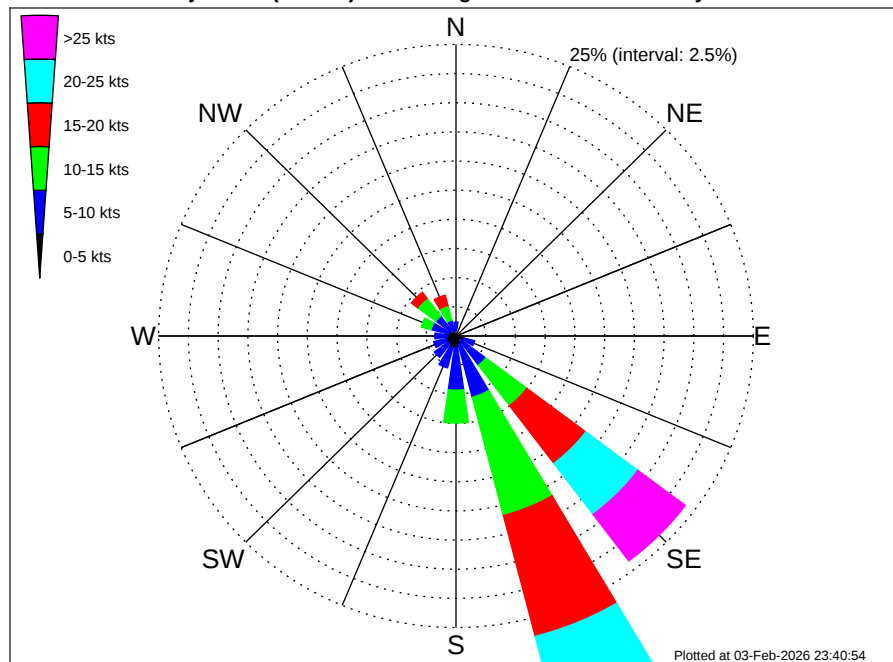
Angola Namibia CRS Oranjemund (BU-OR) Climatological Wind Rose for July: 1979 - 2015
