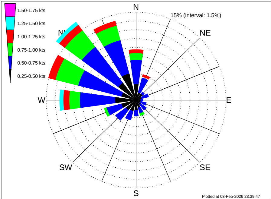
Angola Namibia CRS Oranjemund (BU-OR) Climatological Surface Current Rose for June: 1995 - 2012
