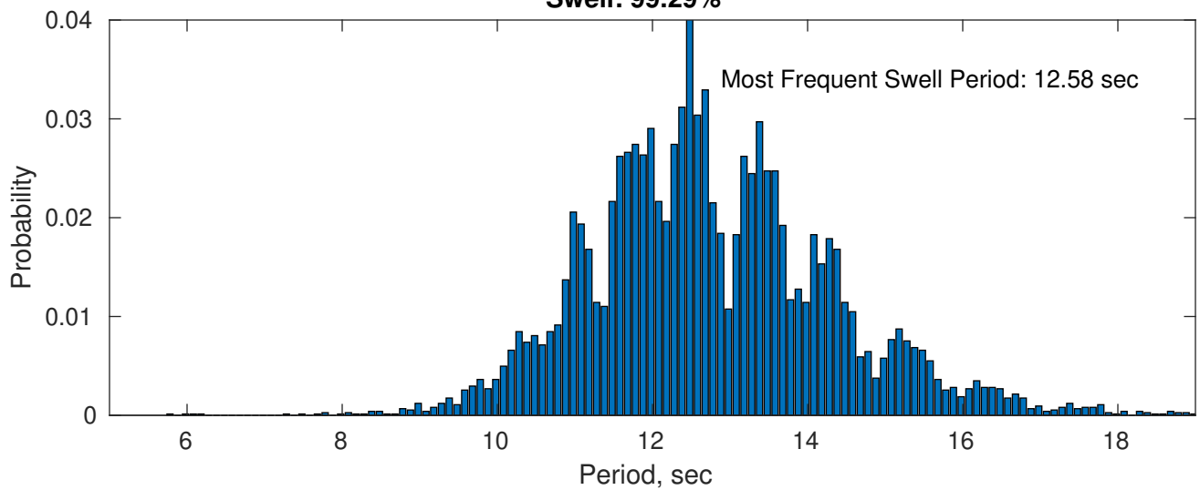
Swell: 99.29%
