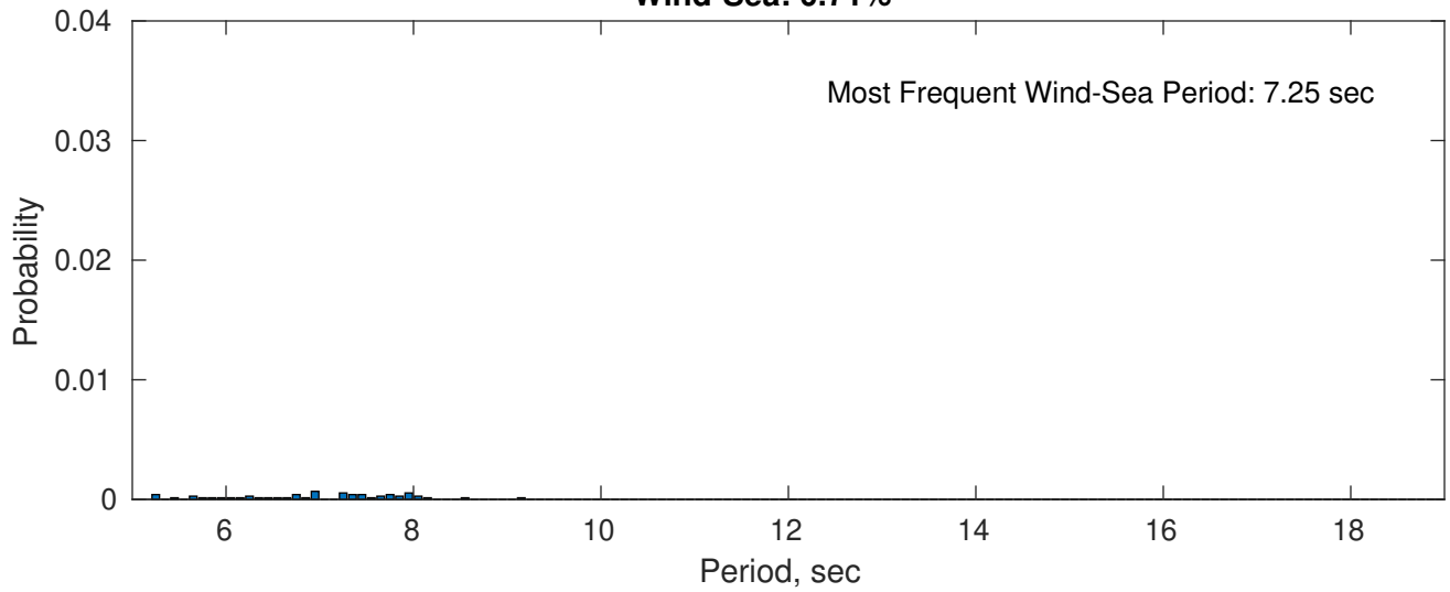
Wind-Sea: 0.71%
