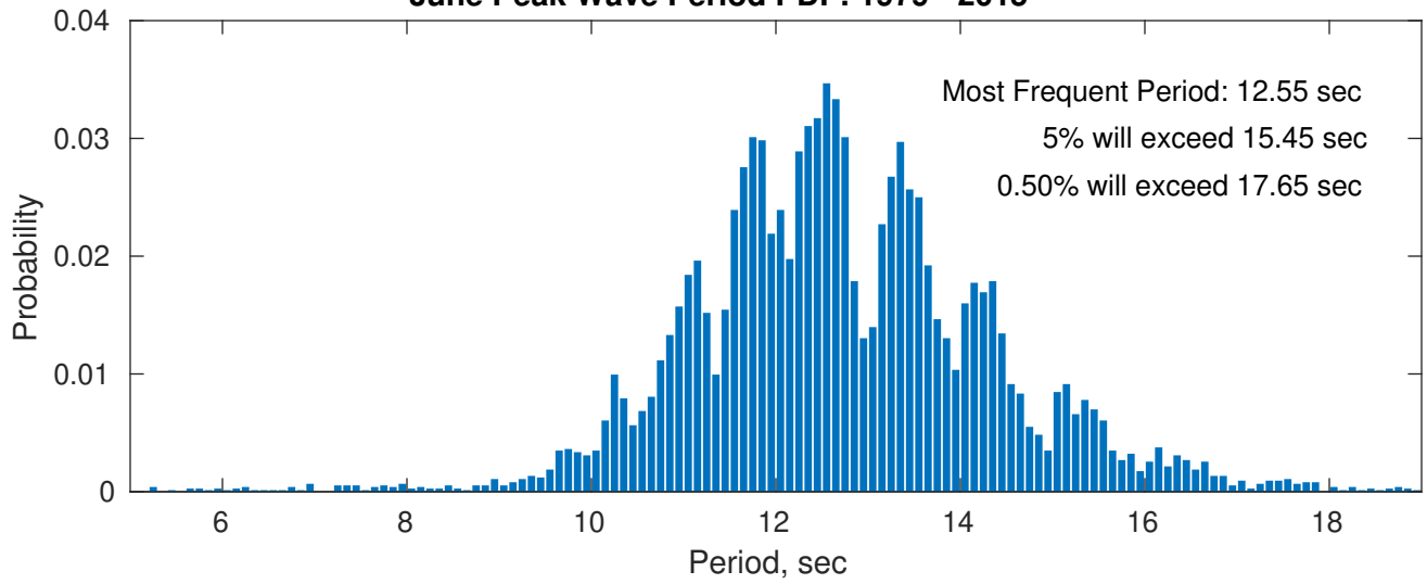
Wind-Sea: 0.71%
