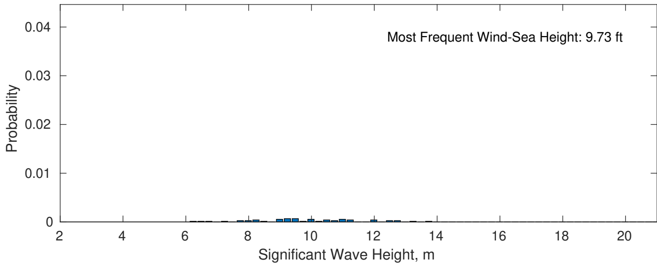
Wind-Sea: 0.71%
