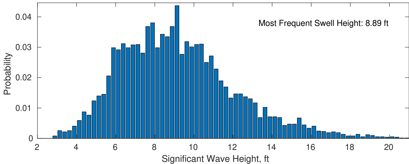
Swell: 99.29%
