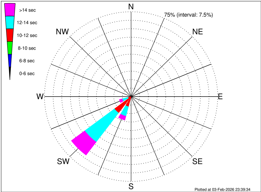
Angola Namibia CRS Oranjemund (BU-OR) Climatological WavePeriod Rose for June: 1979 - 2015
