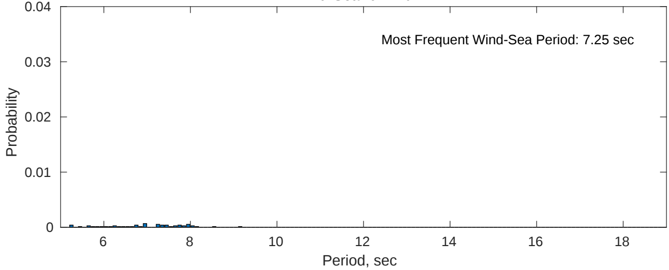
Wind-Sea: 0.71%
