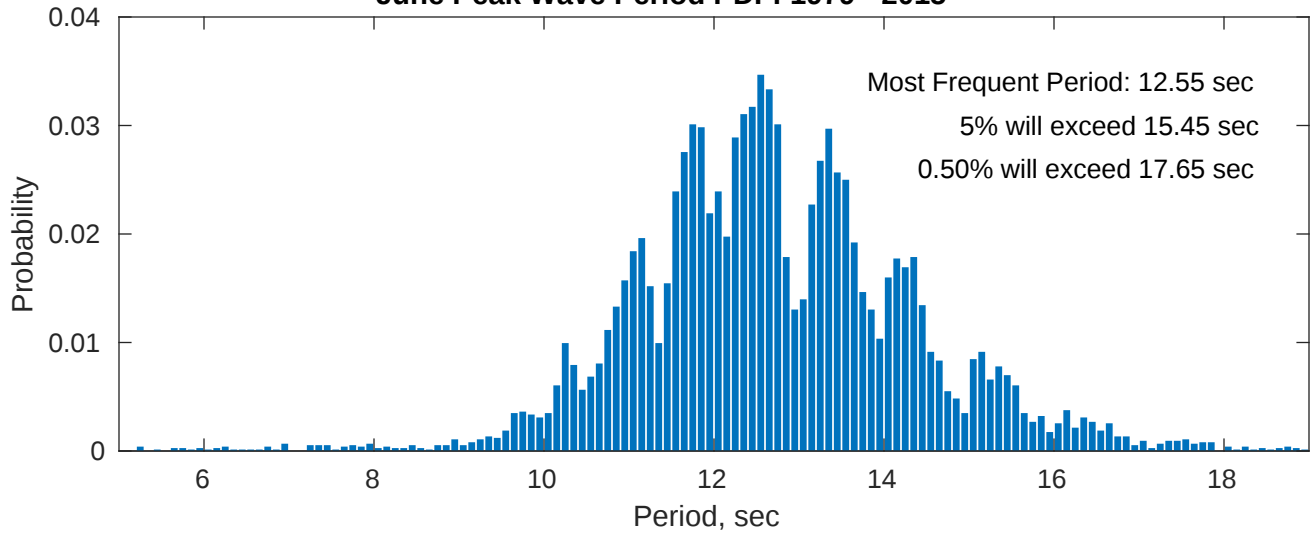
June Peak Wave Period PDF: 1979 - 2015
