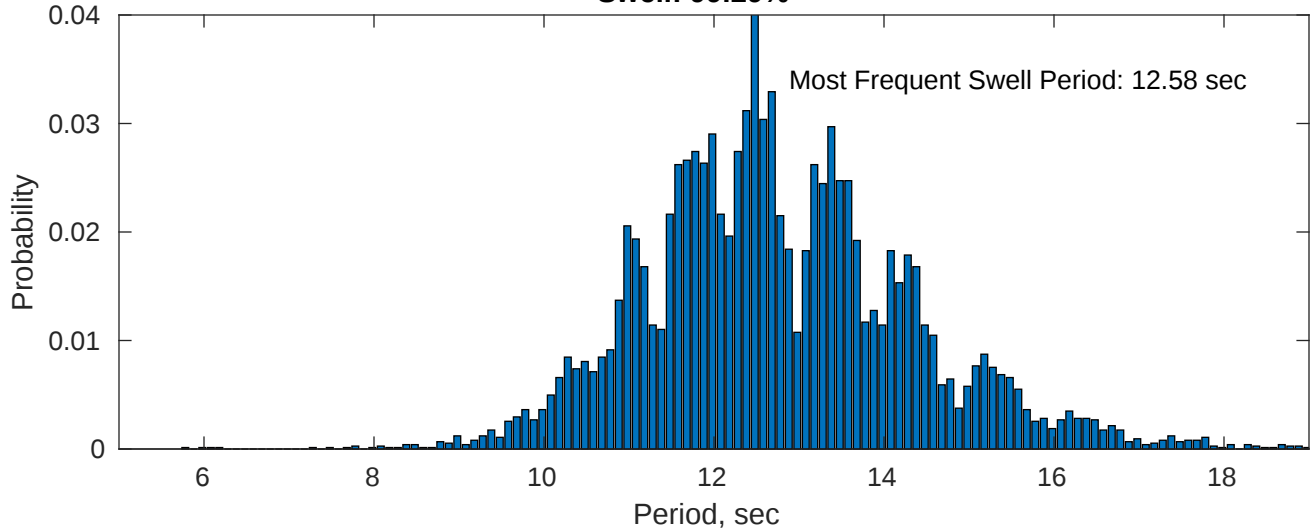
Swell: 99.29%
