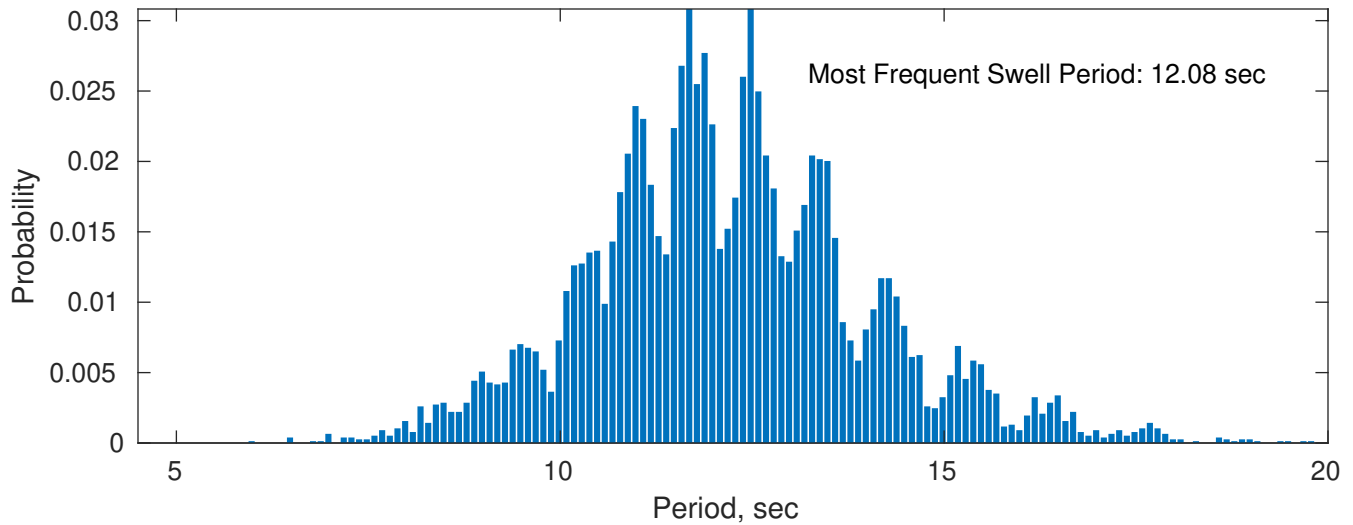
Swell: 93.73%
