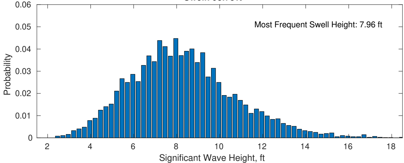
Swell: 93.73%
