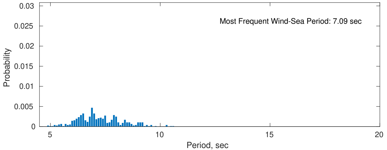
Wind-Sea: 6.27%
