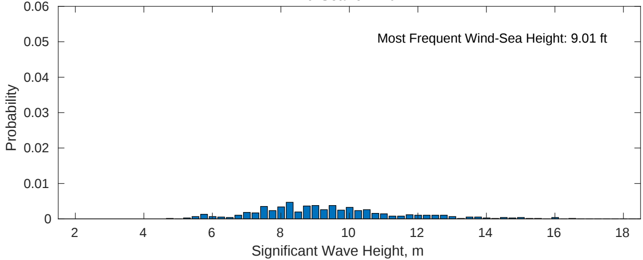
Wind-Sea: 6.27%
