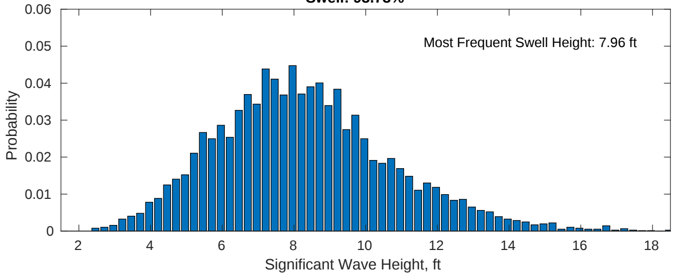
Swell: 93.73%
