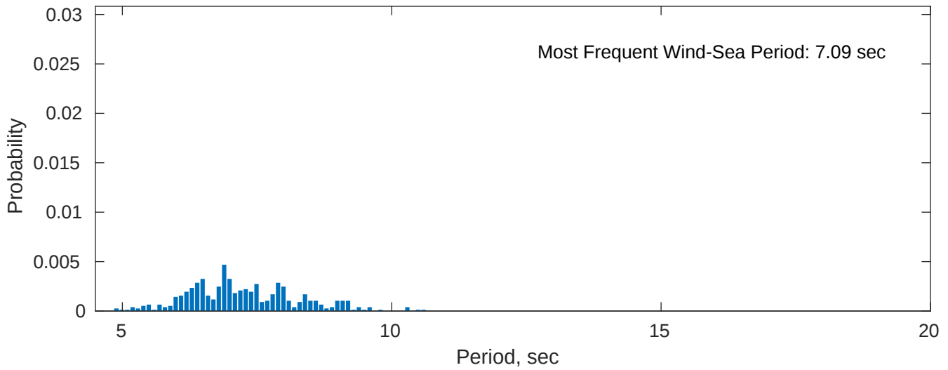
Wind-Sea: 6.27%
