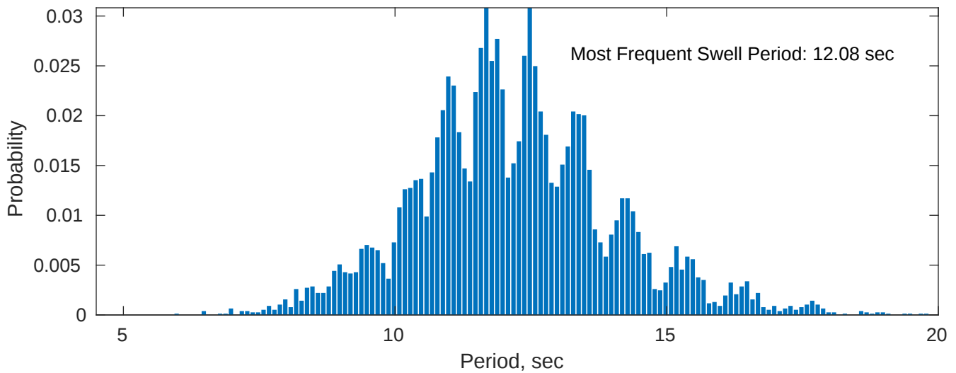
Swell: 93.73%
