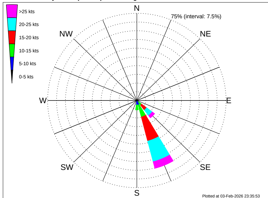
Angola Namibia CRS Oranjemund (BU-OR) Climatological Wind Rose for March: 1979 - 2015
