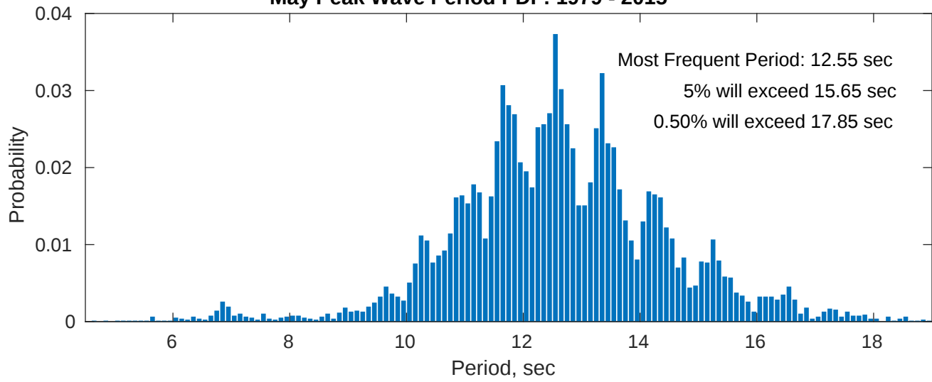
May Peak Wave Period PDF: 1979 - 2015
