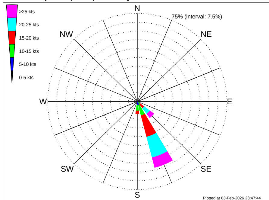
Angola Namibia CRS Oranjemund (BU-OR) Climatological Wind Rose for November: 1979 - 2015
