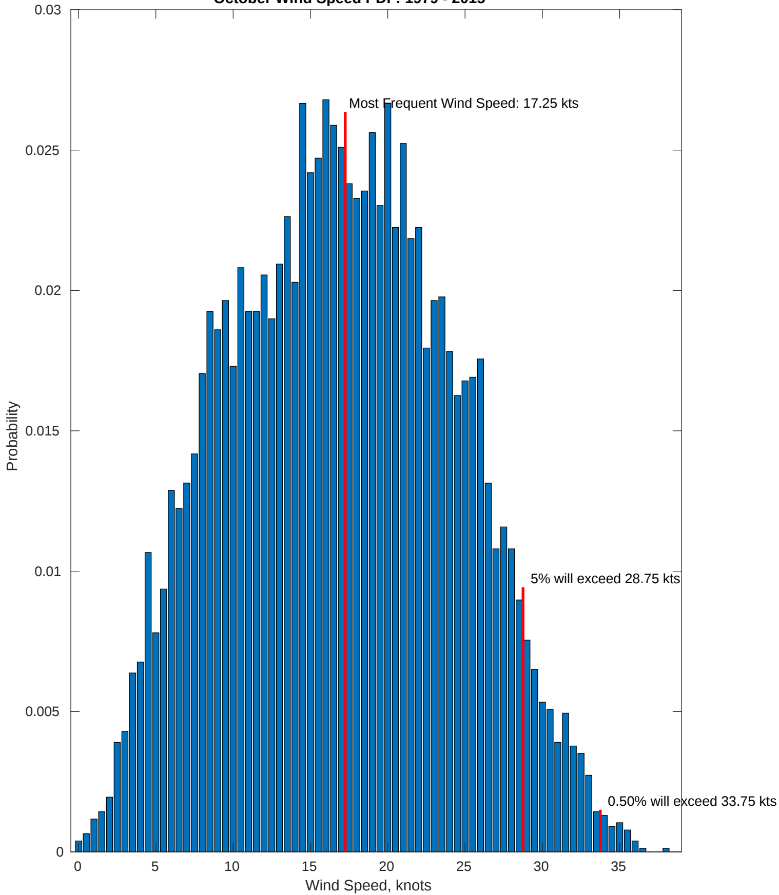
October Wind Speed PDF: 1979 - 2015
