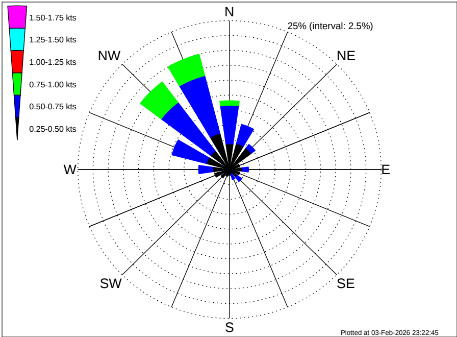
Angola Namibia CRS Swakopmunds (BU-SW) Climatological Surface Current Rose for April: 1995 - 2012
