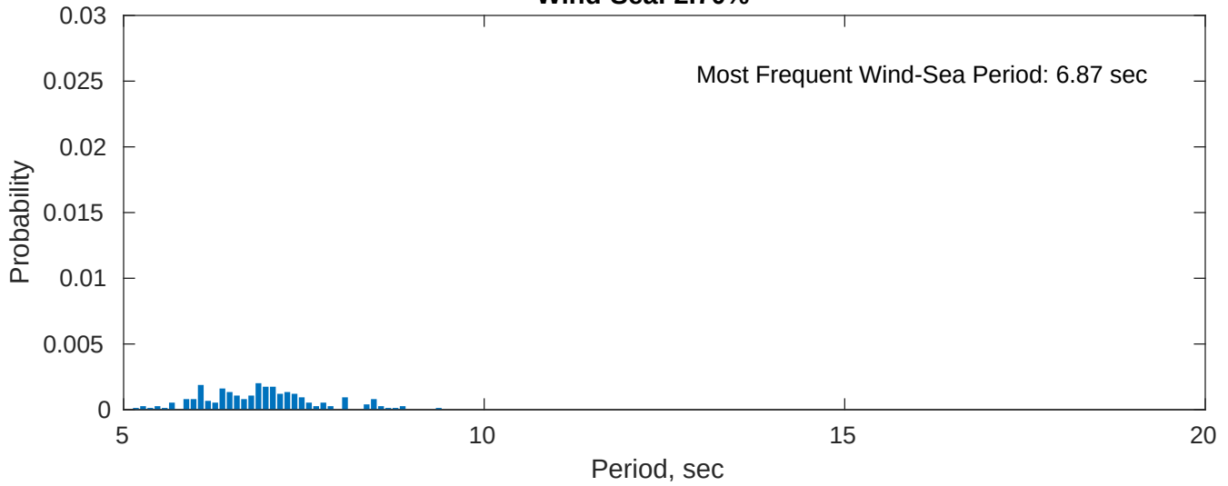
Wind-Sea: 2.70%
