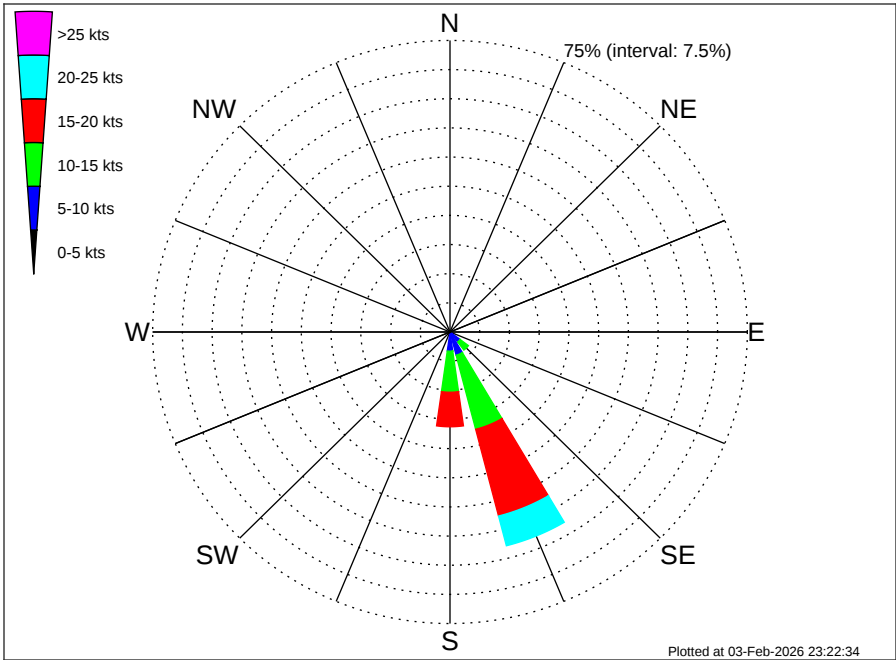
Angola Namibia CRS Swakopmunds (BU-SW) Climatological Wind Rose for April: 1979 - 2015
