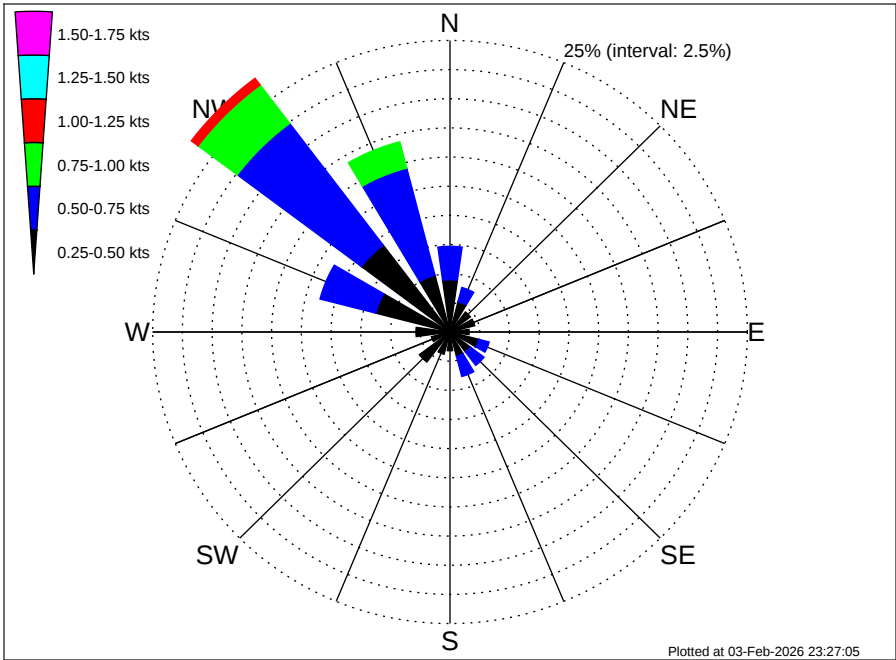
Angola Namibia CRS Swakopmunds (BU-SW) Climatological Surface Current Rose for August: 1995 - 2012
