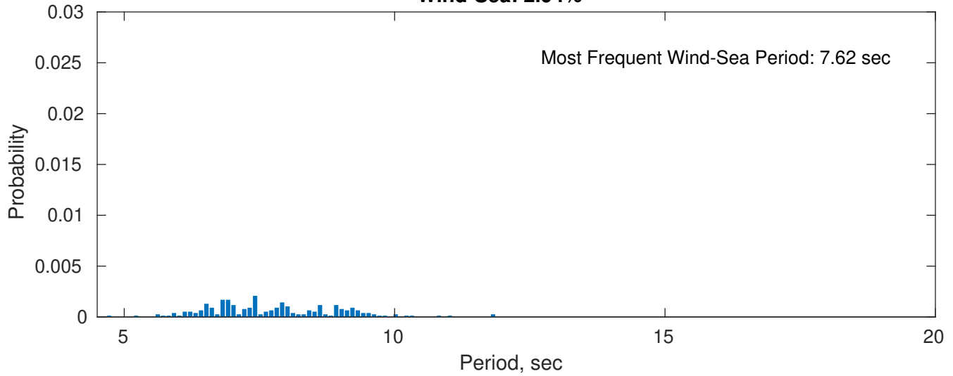
Wind-Sea: 2.94%
