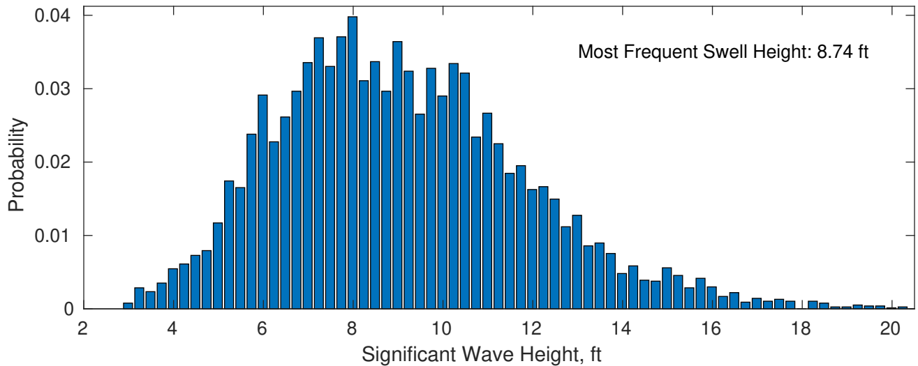
Swell: 97.06%
