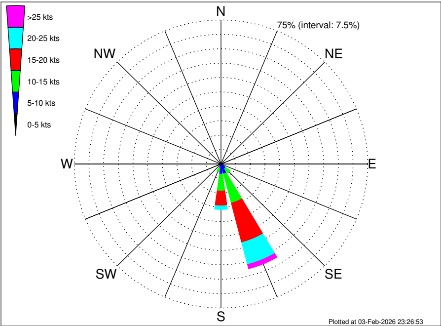
Angola Namibia CRS Swakopmunds (BU-SW) Climatological Wind Rose for August: 1979 - 2015
