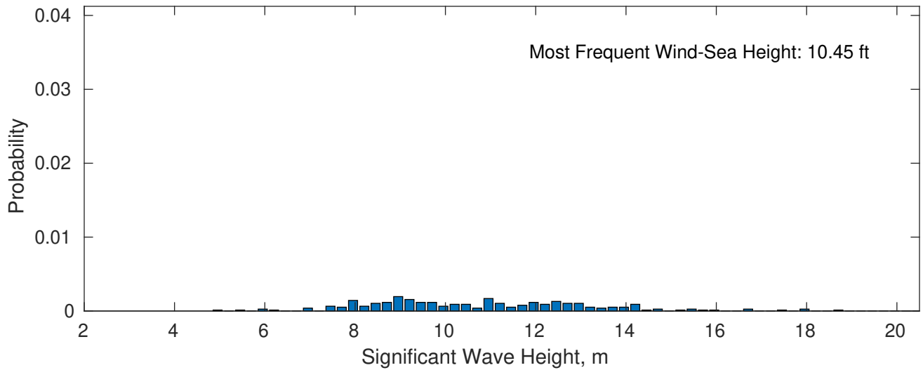
Wind-Sea: 2.94%
