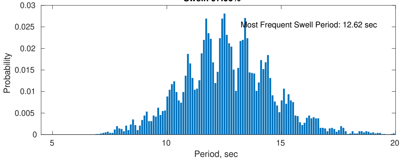
Swell: 97.06%
