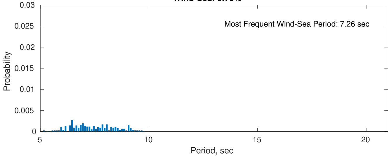
Wind-Sea: 3.73%
