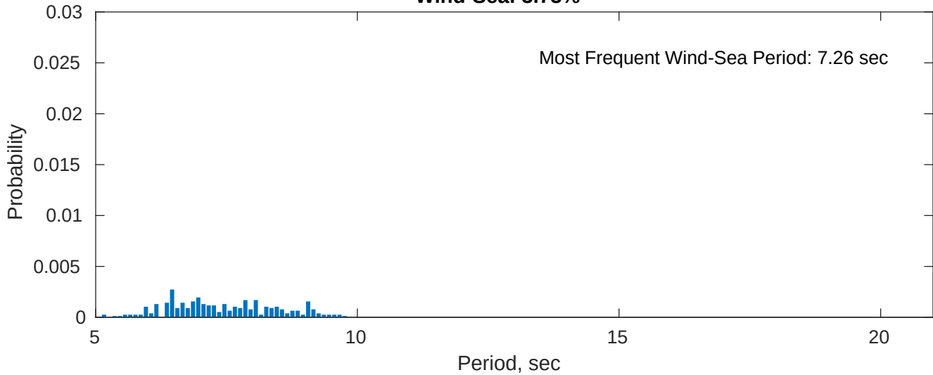
Wind-Sea: 3.73%
