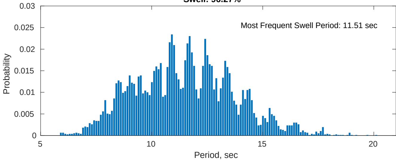
Swell: 96.27%
