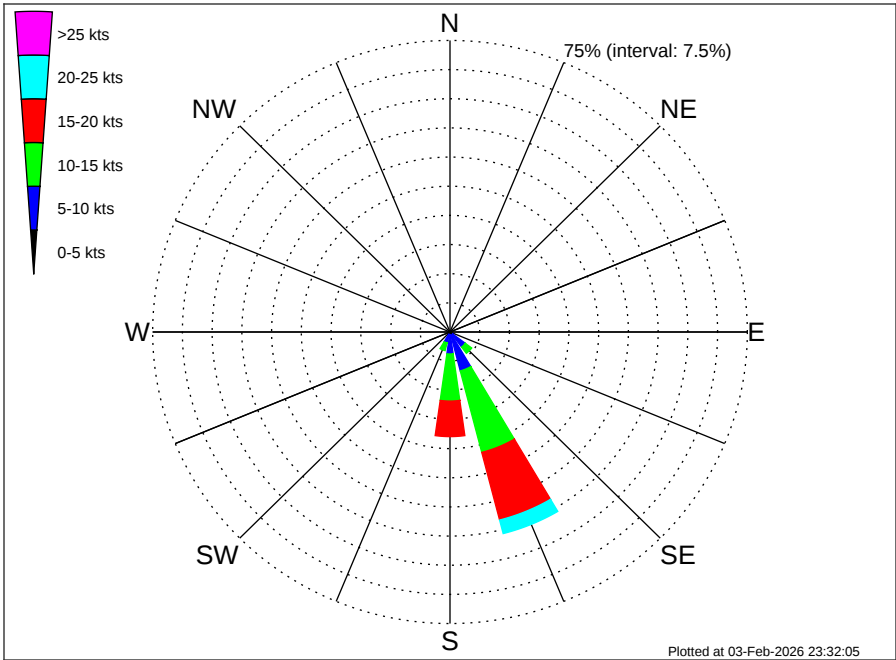
Angola Namibia CRS Swakopmunds (BU-SW) Climatological Wind Rose for December: 1979 - 2015
