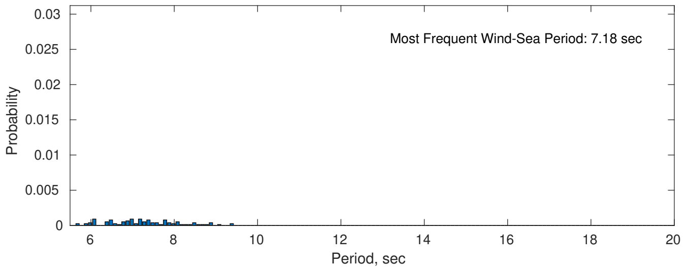
Wind-Sea: 1.29%
