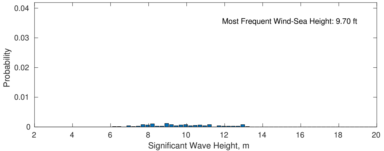
Wind-Sea: 1.29%
