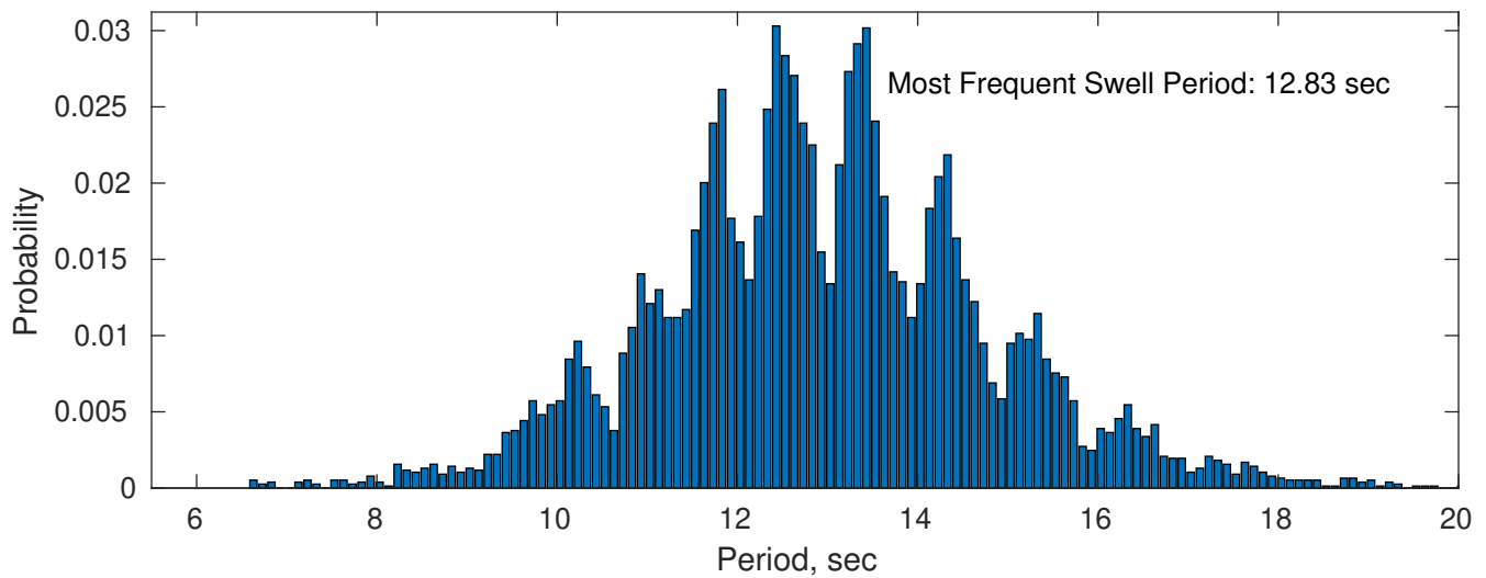
Swell: 98.71%
