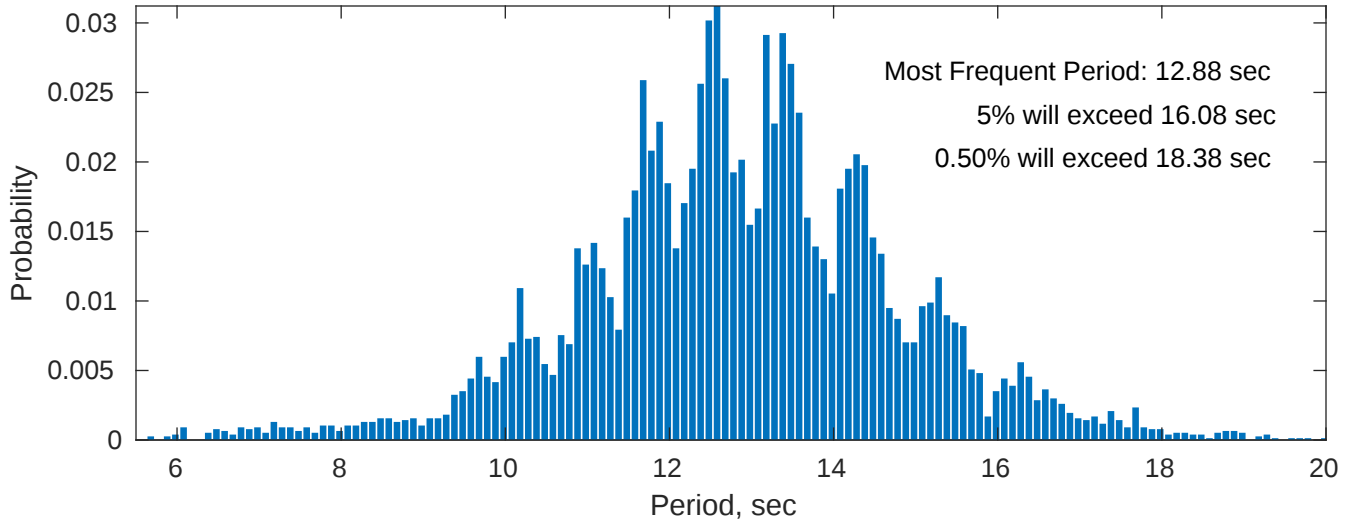
July Peak Wave Period PDF: 1979 - 2015
