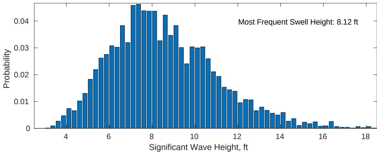
Swell: 98.72%
