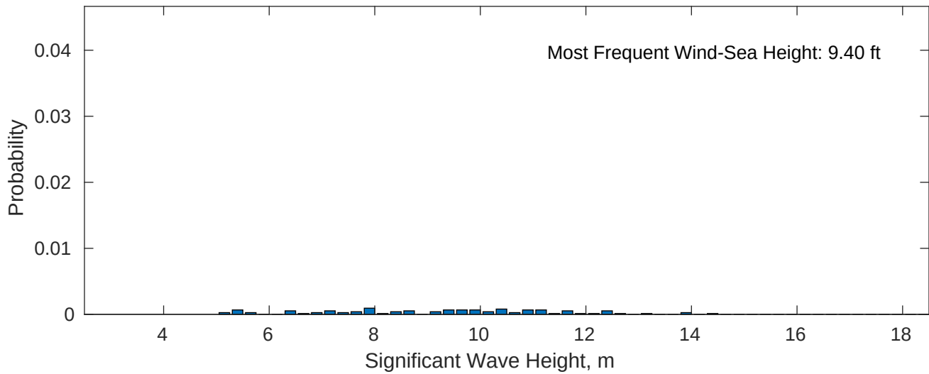
Wind-Sea: 1.28%
