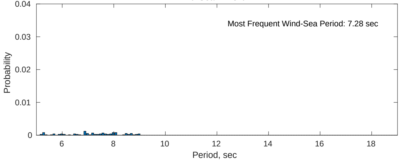
Wind-Sea: 1.28%
