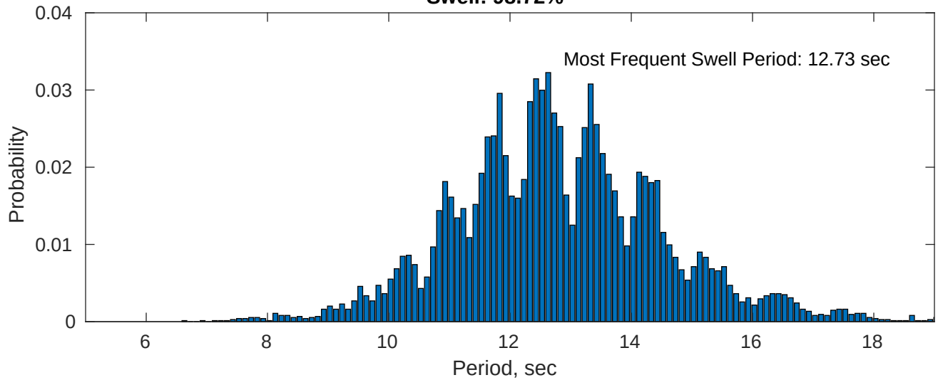
Swell: 98.72%
