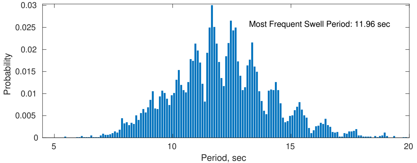
Swell: 97.02%
