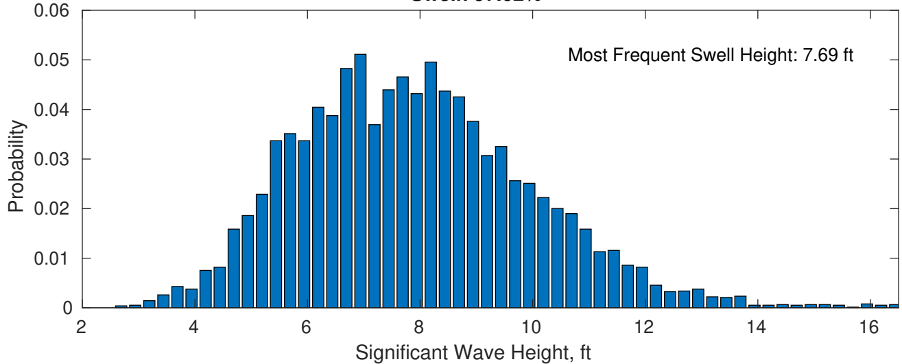
Swell: 97.02%
