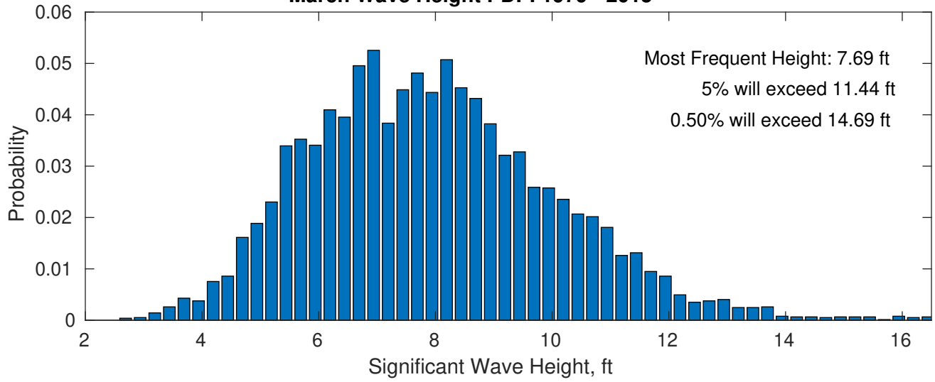
Wind-Sea: 2.98%
