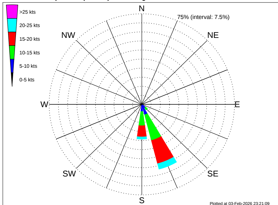
Angola Namibia CRS Swakopmunds (BU-SW) Climatological Wind Rose for March: 1979 - 2015
