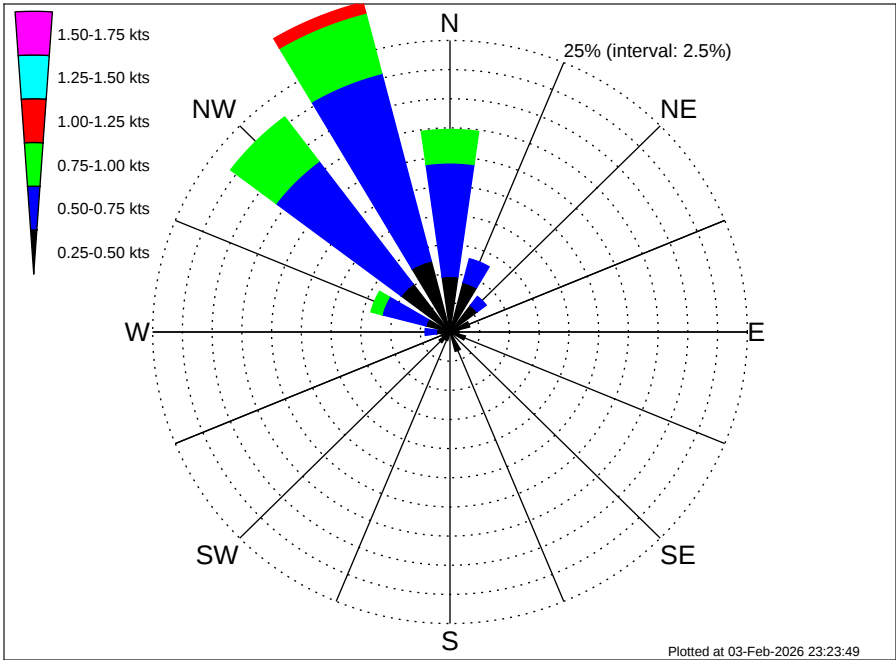
Angola Namibia CRS Swakopmunds (BU-SW) Climatological Surface Current Rose for May: 1995 - 2012
