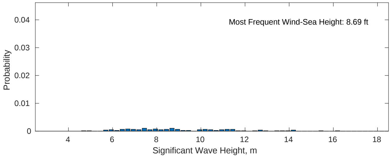
Wind-Sea: 1.55%
