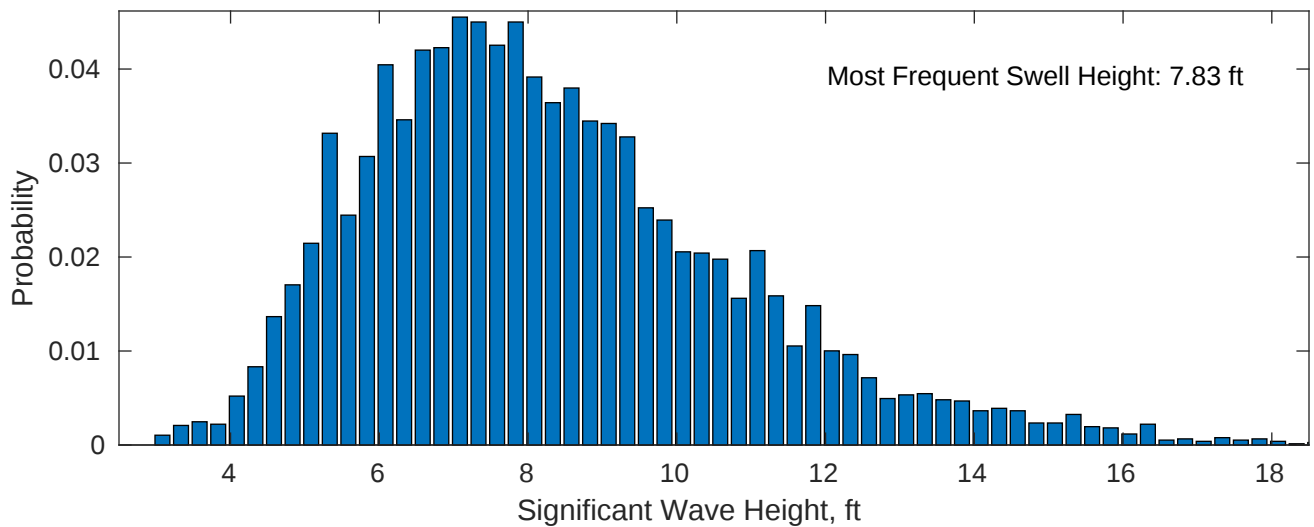
Swell: 98.45%
