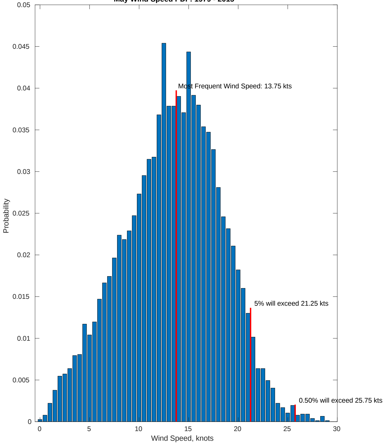
May Wind Speed PDF: 1979 - 2015
