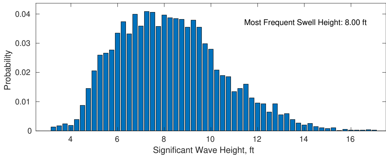
Swell: 93.17%
