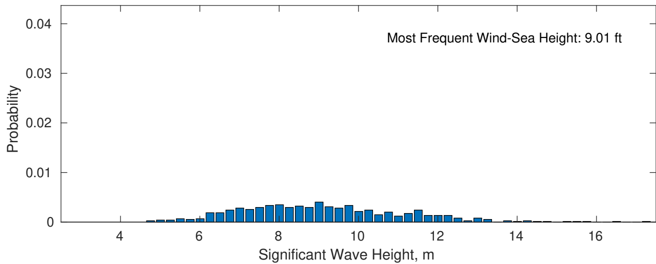
Wind-Sea: 6.83%
