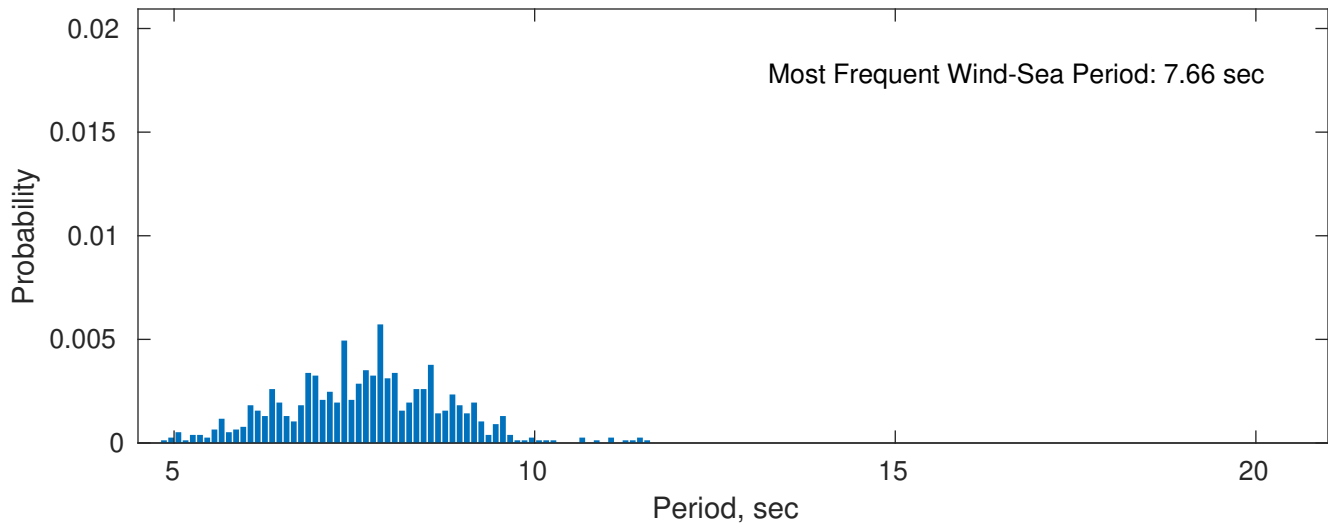
Wind-Sea: 9.05%
