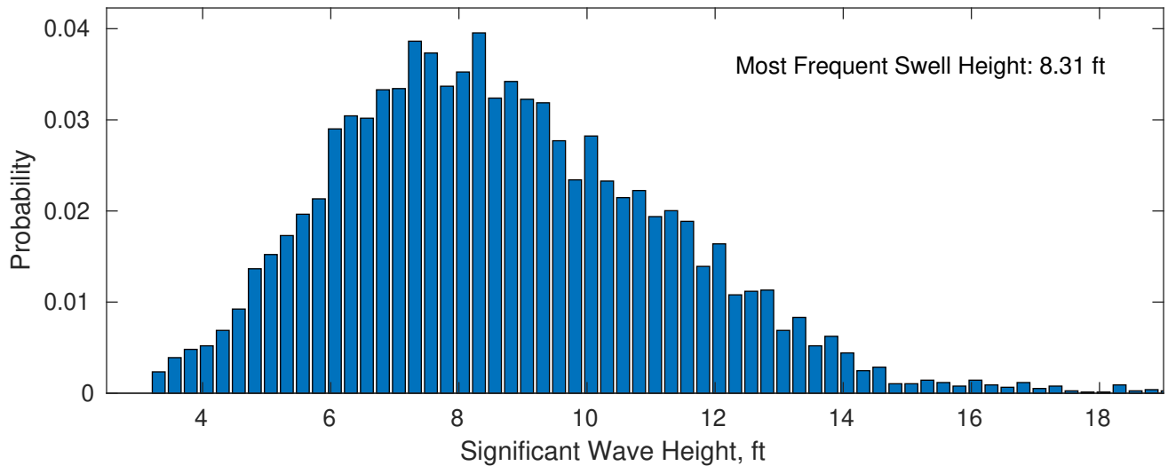
Swell: 90.95%
