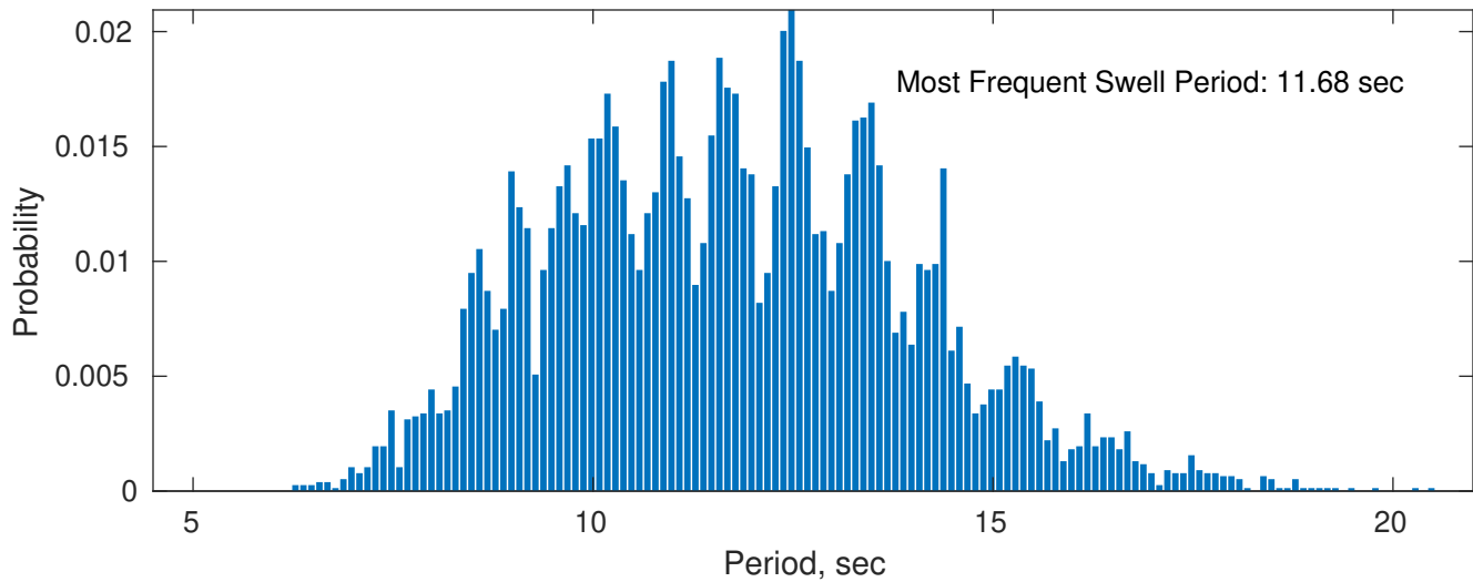
Swell: 90.95%
