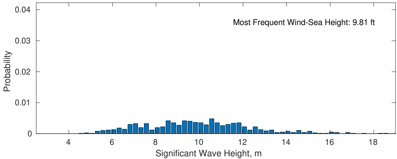
Wind-Sea: 9.05%
