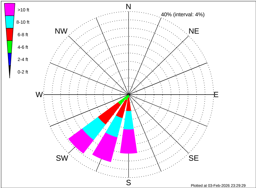
Angola Namibia CRS Swakopmunds (BU-SW) Climatological WaveHeight Rose for October: 1979 - 2015
