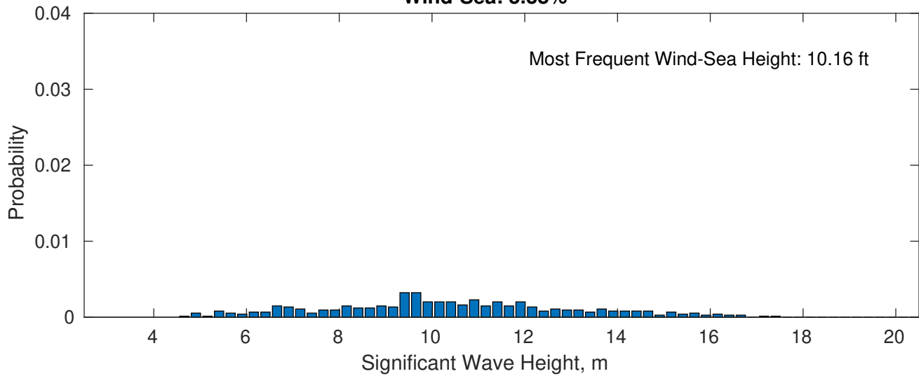
Wind-Sea: 5.38%
