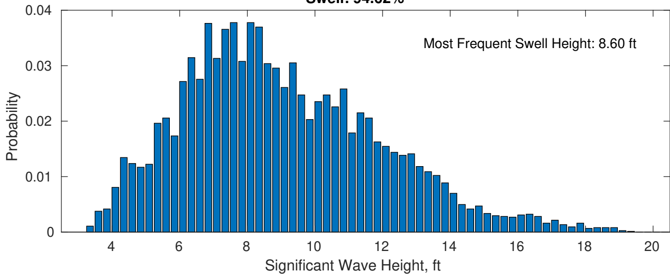
Swell: 94.62%
