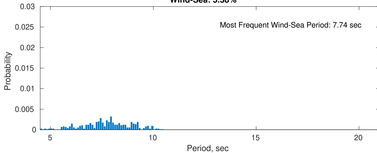
Wind-Sea: 5.38%
