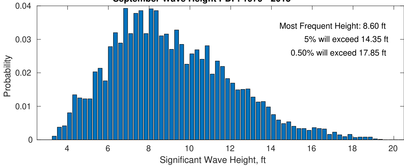
Wind-Sea: 5.38%
