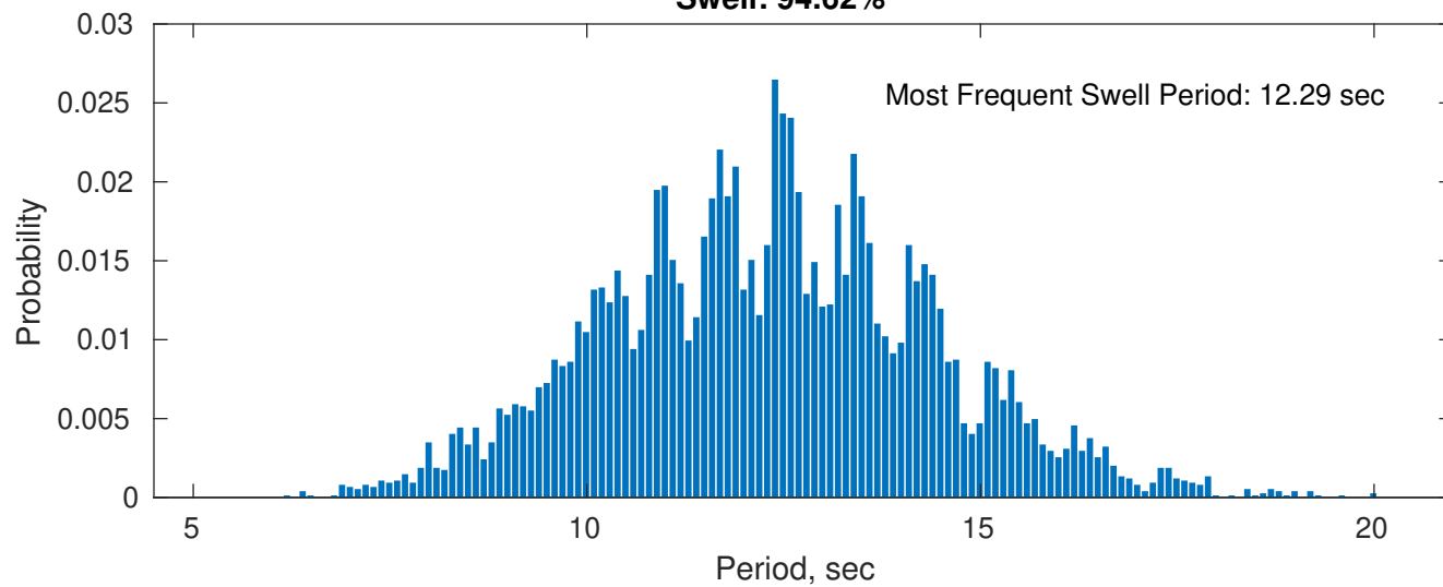
Swell: 94.62%
