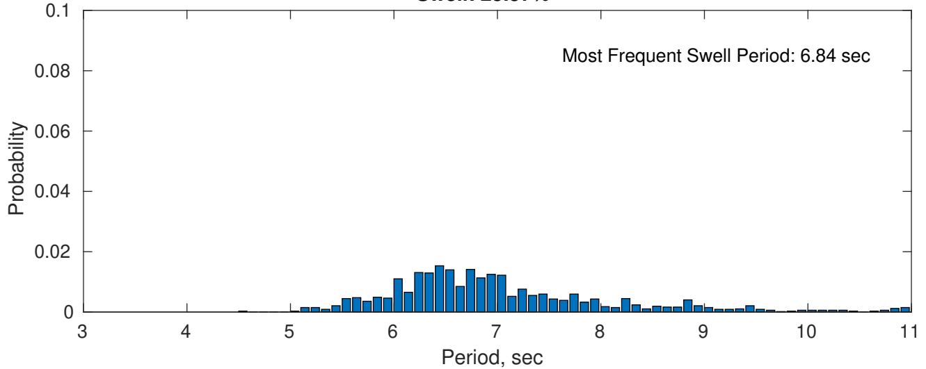
Swell: 25.57%
