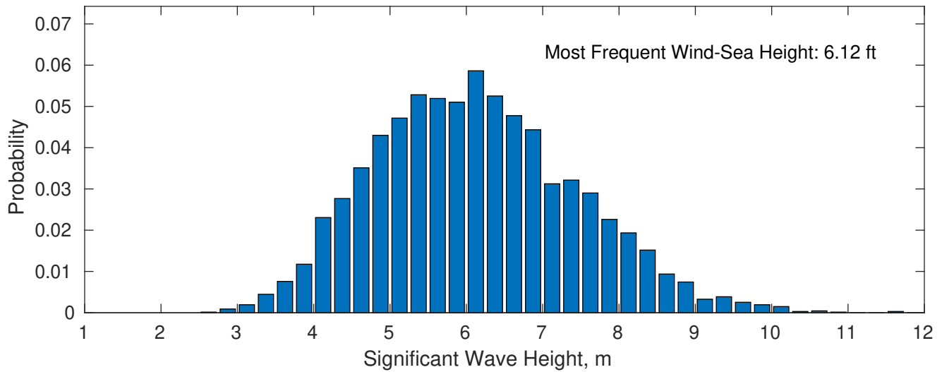
Wind-Sea: 74.43%
