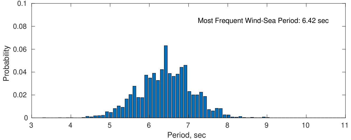
Wind-Sea: 74.43%
