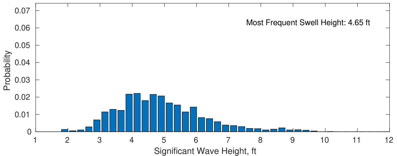
Swell: 25.57%
